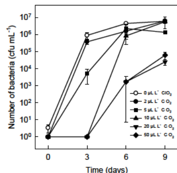
Fig. 1. Number of bacteria in Gerbera vase water treated with various ClO 2 concentrations.
